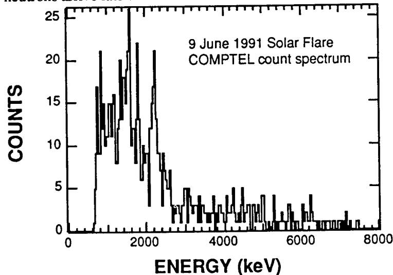
FIG. 2: The raw telescope mode count spectrum from the 9 June 1991 solar flare.
