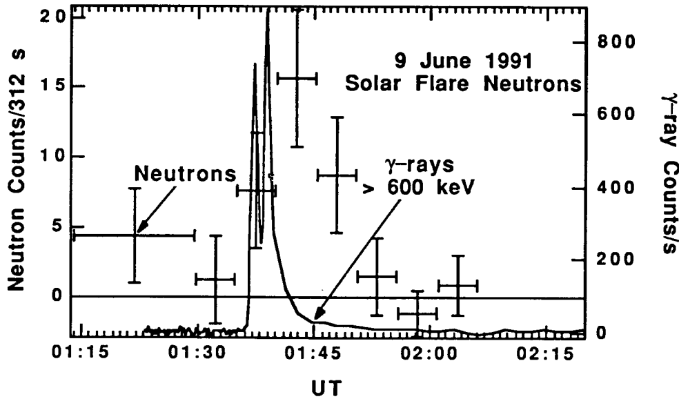
FIG. 3: Neutron and \gamma -ray emission-time profiles for the 9 June 1991 solar flare, plotted at the time corresponding to a photon arrival time.
