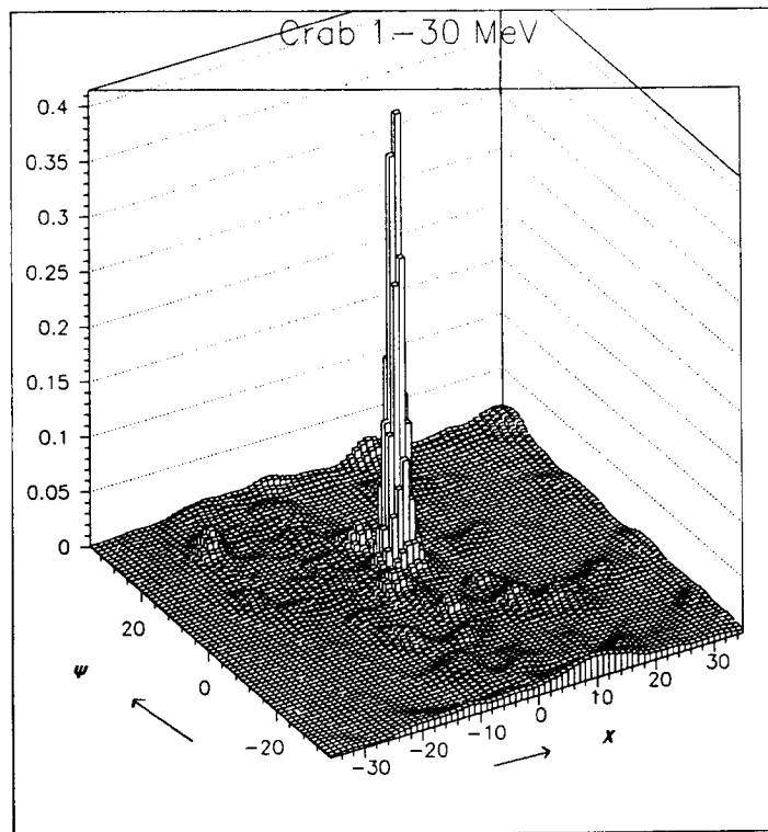
Fig. 2. Maximum Entropy image of the Anticenter region showing the Crab. Coordinates are in the telescope system. Crab is at \chi = 0.1 , \psi = 6.4 . The position of Geminga is at \chi = 8.2 , \psi = 5.6 .
