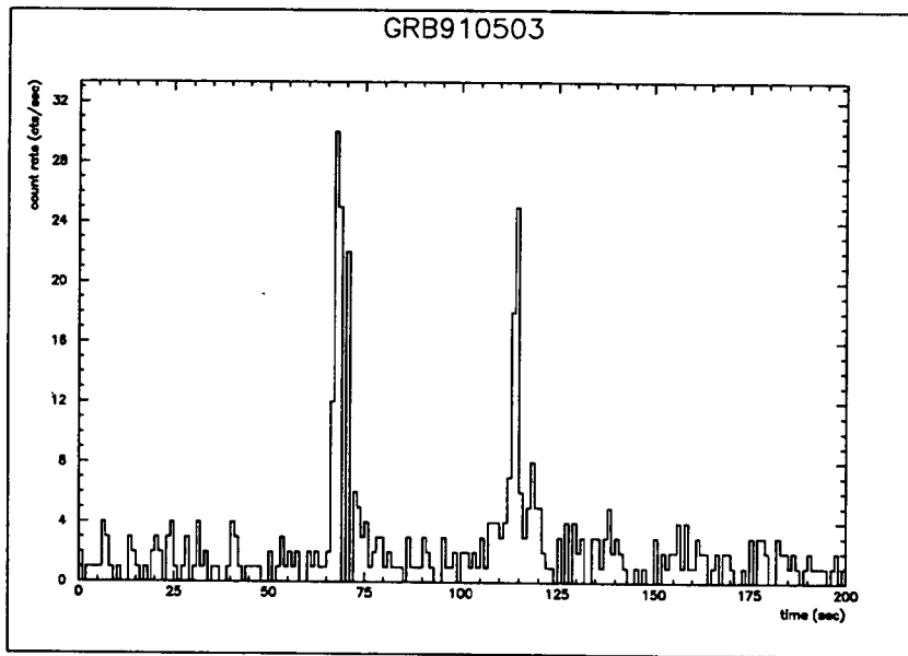
Fig. 5. Time Profile of GRB 910503 as measured in the COMPTEL telescope mode (1-20 MeV).
